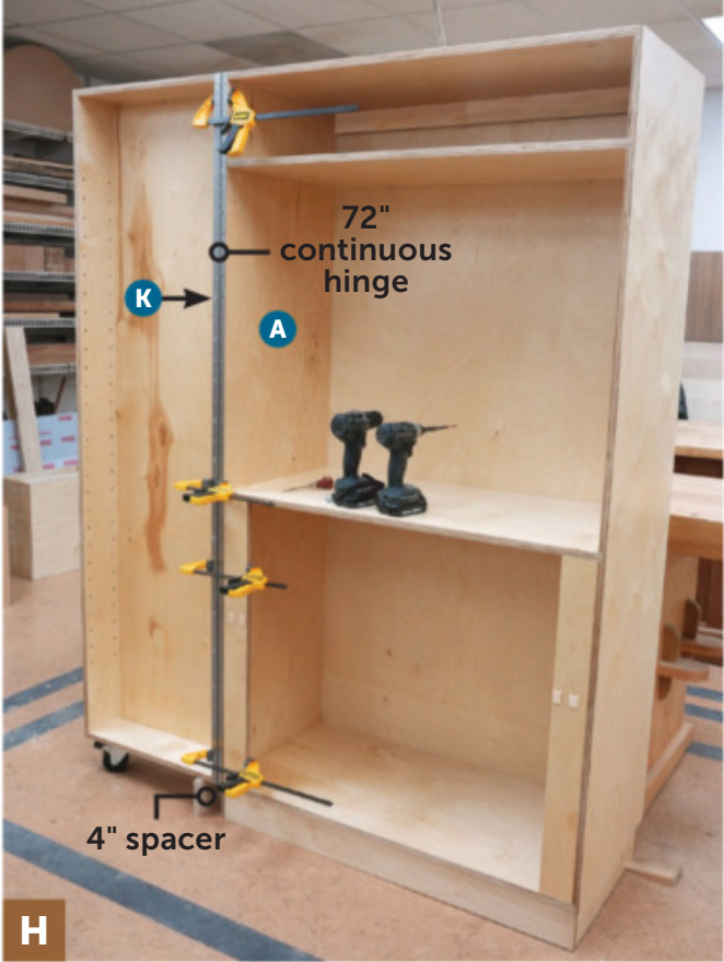
Support the hinge side of the door with a 4" spacer. Then clamp the door to the cabinet with a 1/8" spacer (thickness of the hinge barrel) in between. Screw the hinge to the cabinet side (A) and door side (K).
