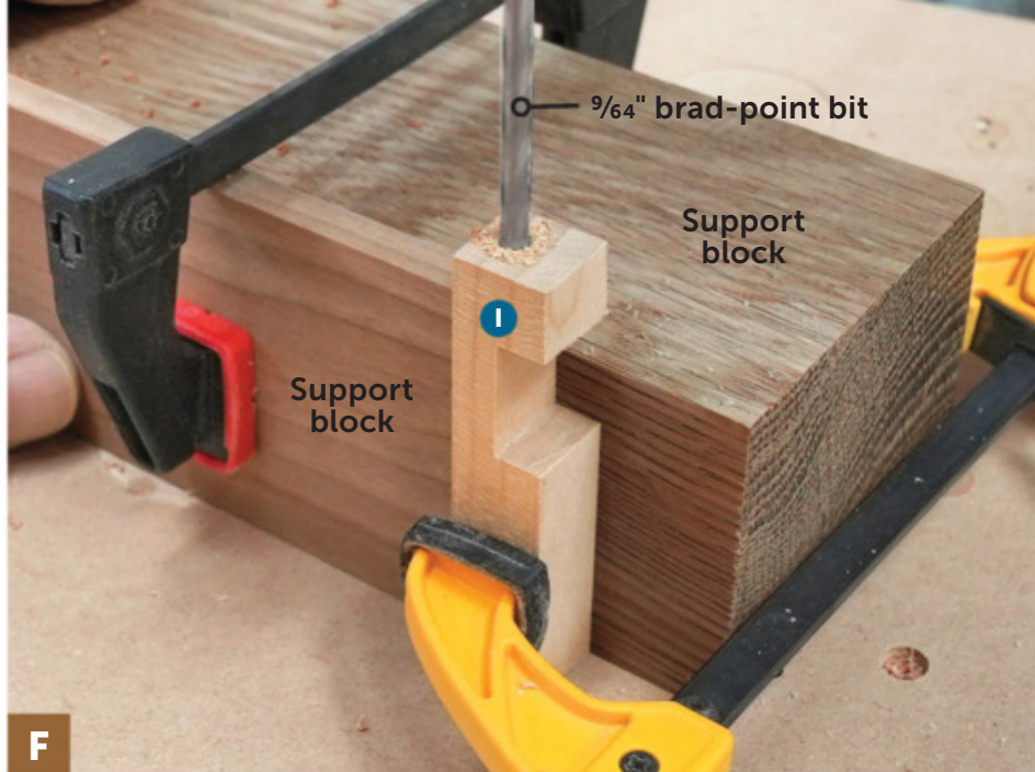
Use a pair of support blocks to hold the tongue blank plumb, square, and vertical while drilling a hole in the end. A \frac{9}{64} " brad-point bit makes a clean hole in the end grain, without wandering.
