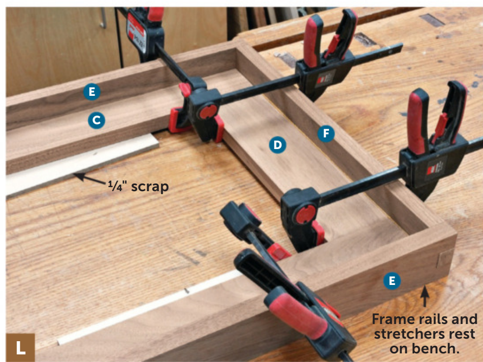
L Scrap material lifts the seat support (C/D) to create a lower lip. Glue a frame rail (E) to a frame stretcher (F), then glue this assembly to the seat support. Add the remaining stretcher and rail.
